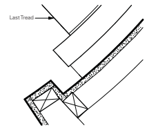
Detail 3 Stair Plan at 13th Floor - Last tread
