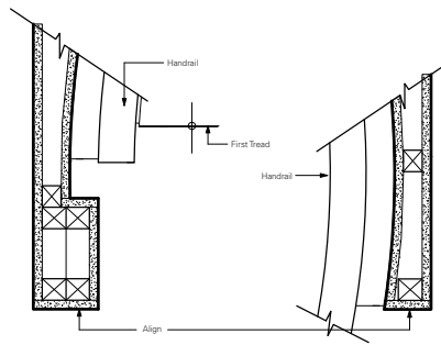
Detail 1 Plan Detail First Level
